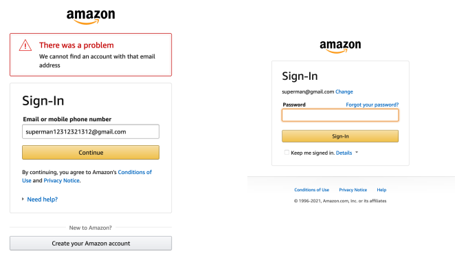
Fig. 1. Enumerating when the username doesn't exist, by this method you can see if superman@gmail.com exists, it will not show the error message shown in the first figure
